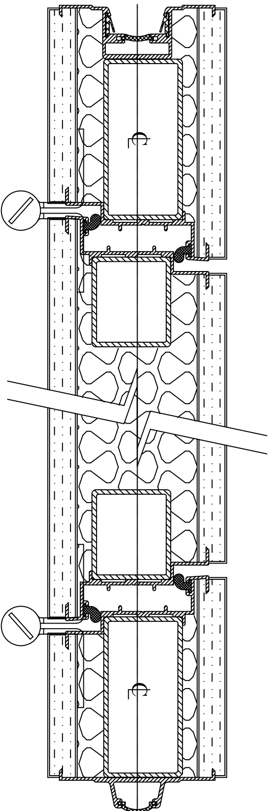
PLAN SECTION at DOUBLE DOOR PANEL (SE Wicket Door)
